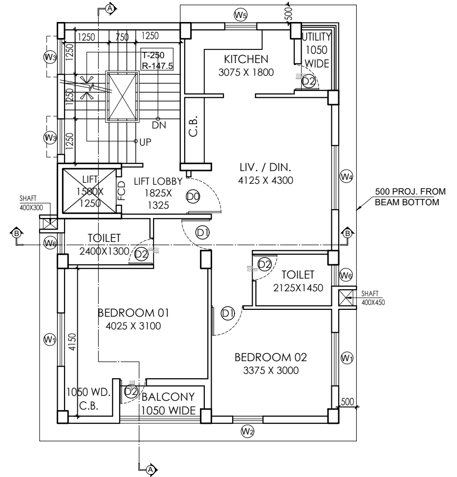
TYPICAL (1ST TO 4TH) FLOOR PLAN SCALE 1:100
